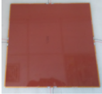
BA Model
