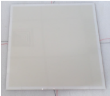
BA Model
