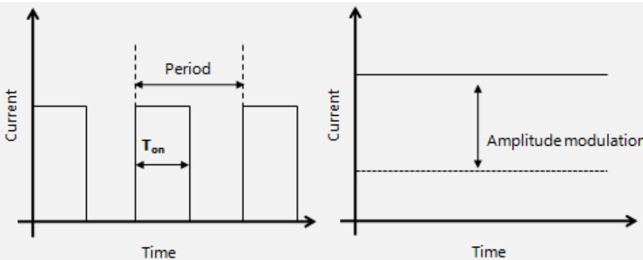
Fig 1. PWM Driver (Recom)
